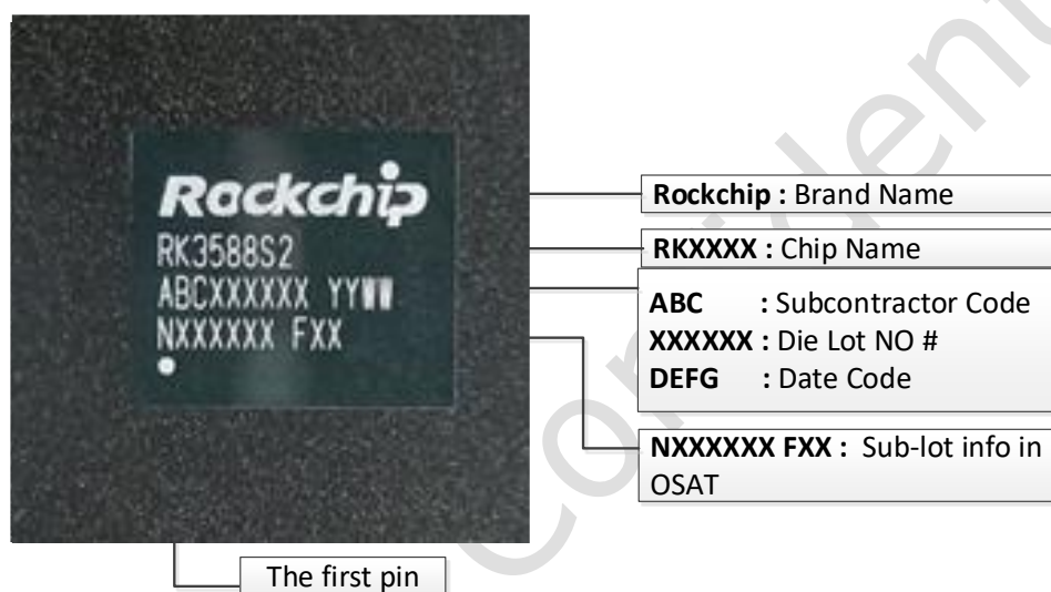
Fig.2-1 Package definition
